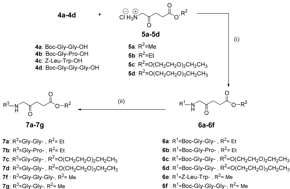
Scheme 1. Chemical syntheses.
